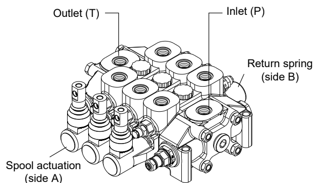
SECTIONAL VALVES WITH RIGHT INLET
