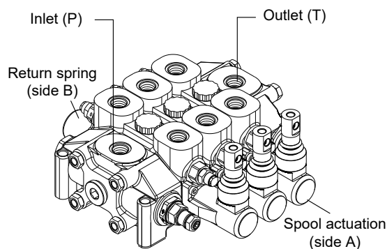
SECTIONAL VALVES WITH LEFT INLET
